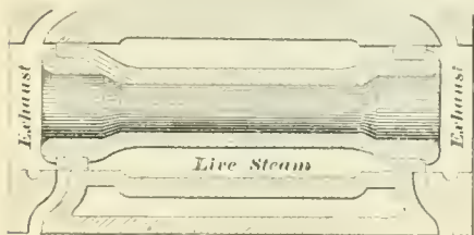
FIG. 7. CENTRAL ADMISSION.
